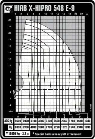
Lastdiagram HIAB X-HIPRO 548 E-9
