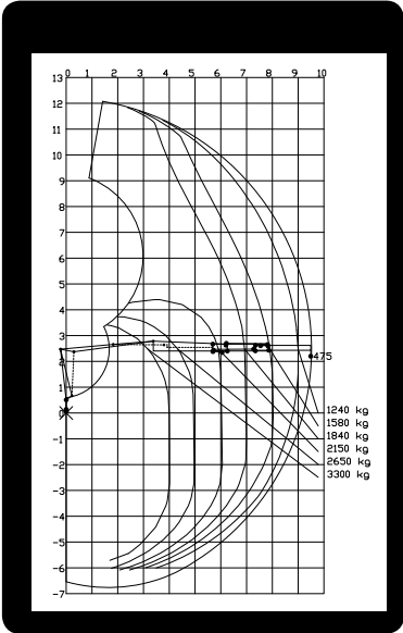
Load diagram 1400Z95
