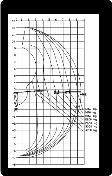
Load diagram 1500Z95
