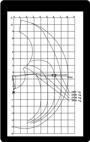
Load diagram 1400Z80
