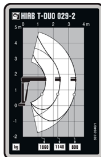
Lastdiagram HIAB T-DUO 029-2
