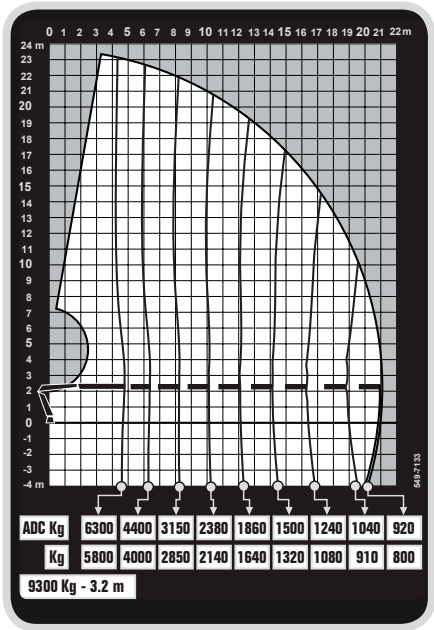
Lastdiagram HIAB X-HIPRO 352 E-8
