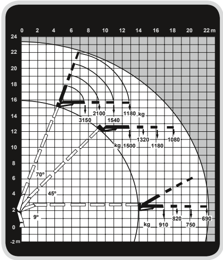
Lastdiagram HIAB X-HIPRO 352 E-5 JIB 100X-3
