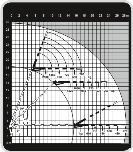
Lastdiagram HIAB X-HIPRO 352 E-6 JIB 70X-4
